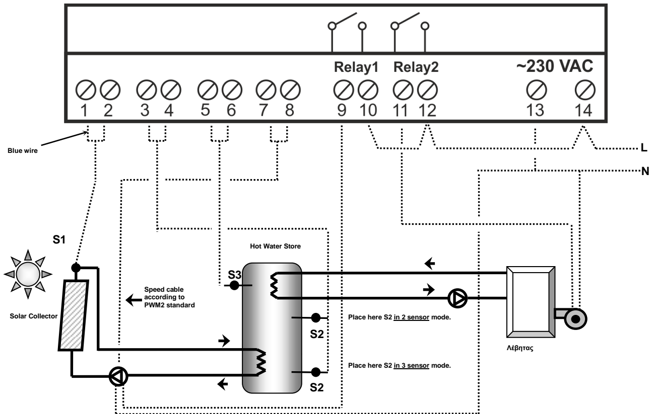
Figure 1 Wiring Diagram
