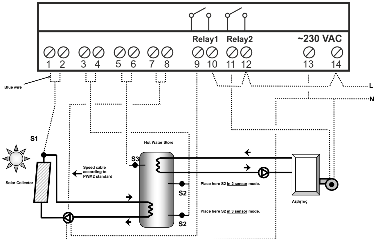
Figure 1 Wiring Diagram
