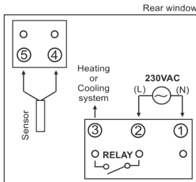
Figure 3 Electrical connections
